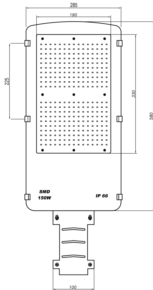
View front
