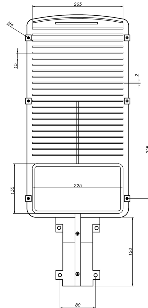
View back
