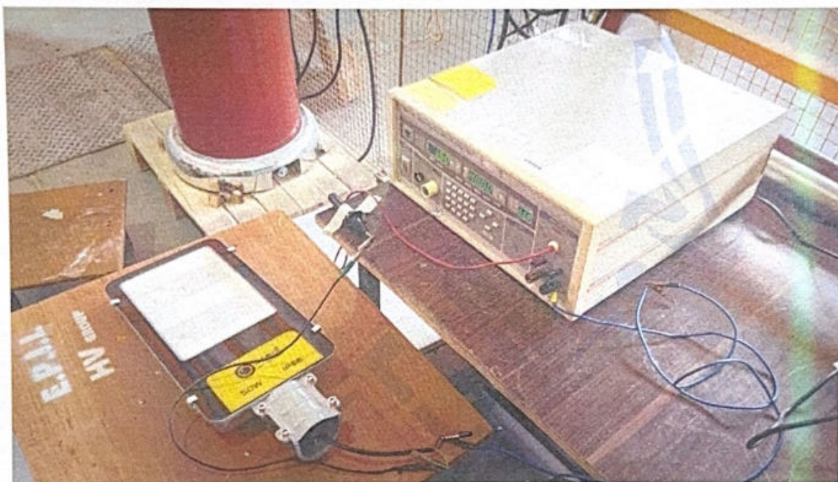
Figure 4: EUT under AC voltage test
