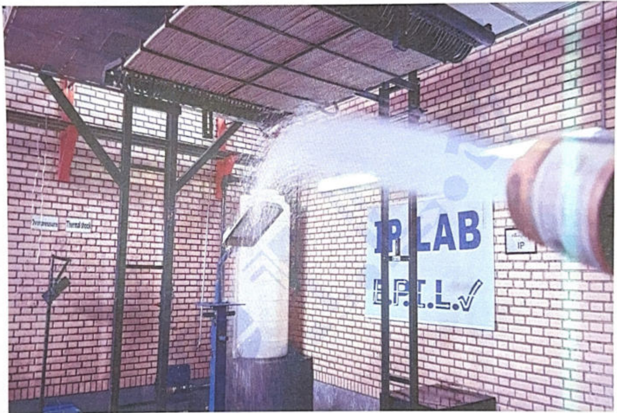
Figure 3: EUT under IPX6
