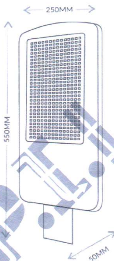
Figure 5: Dimension
