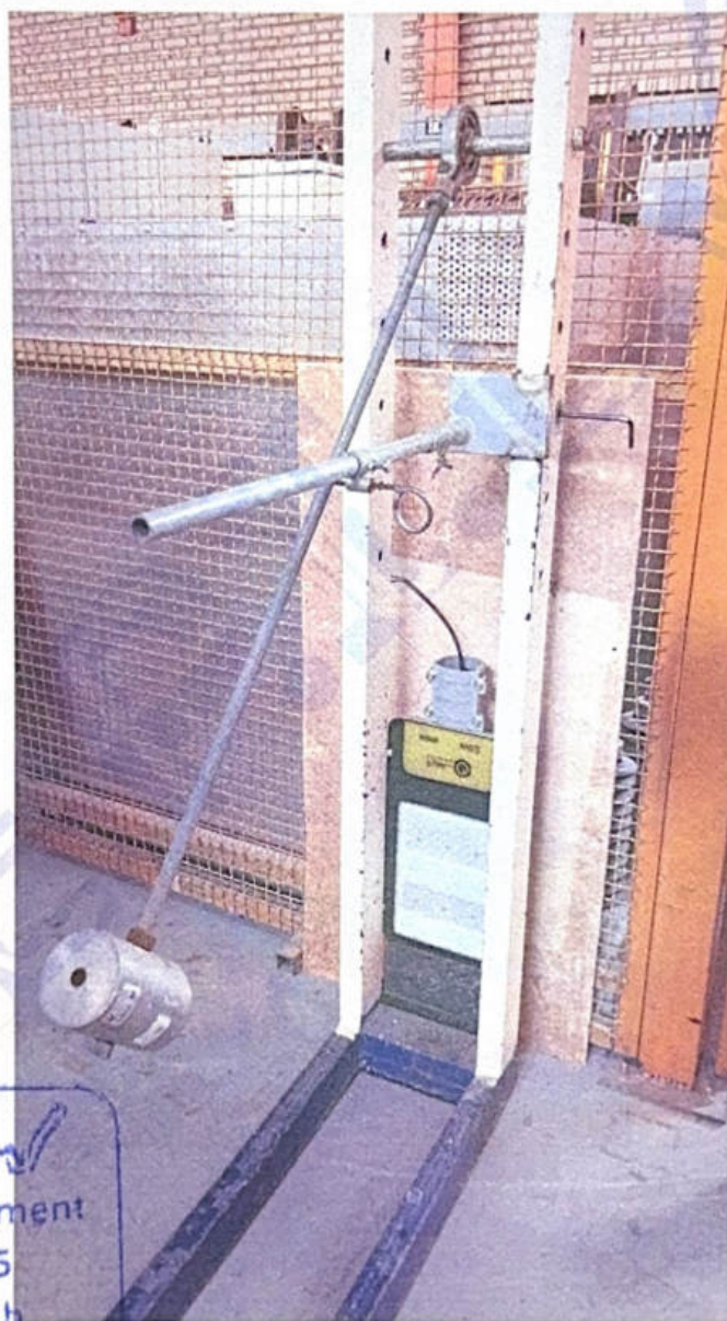
Figure 1: EUT under IK10
