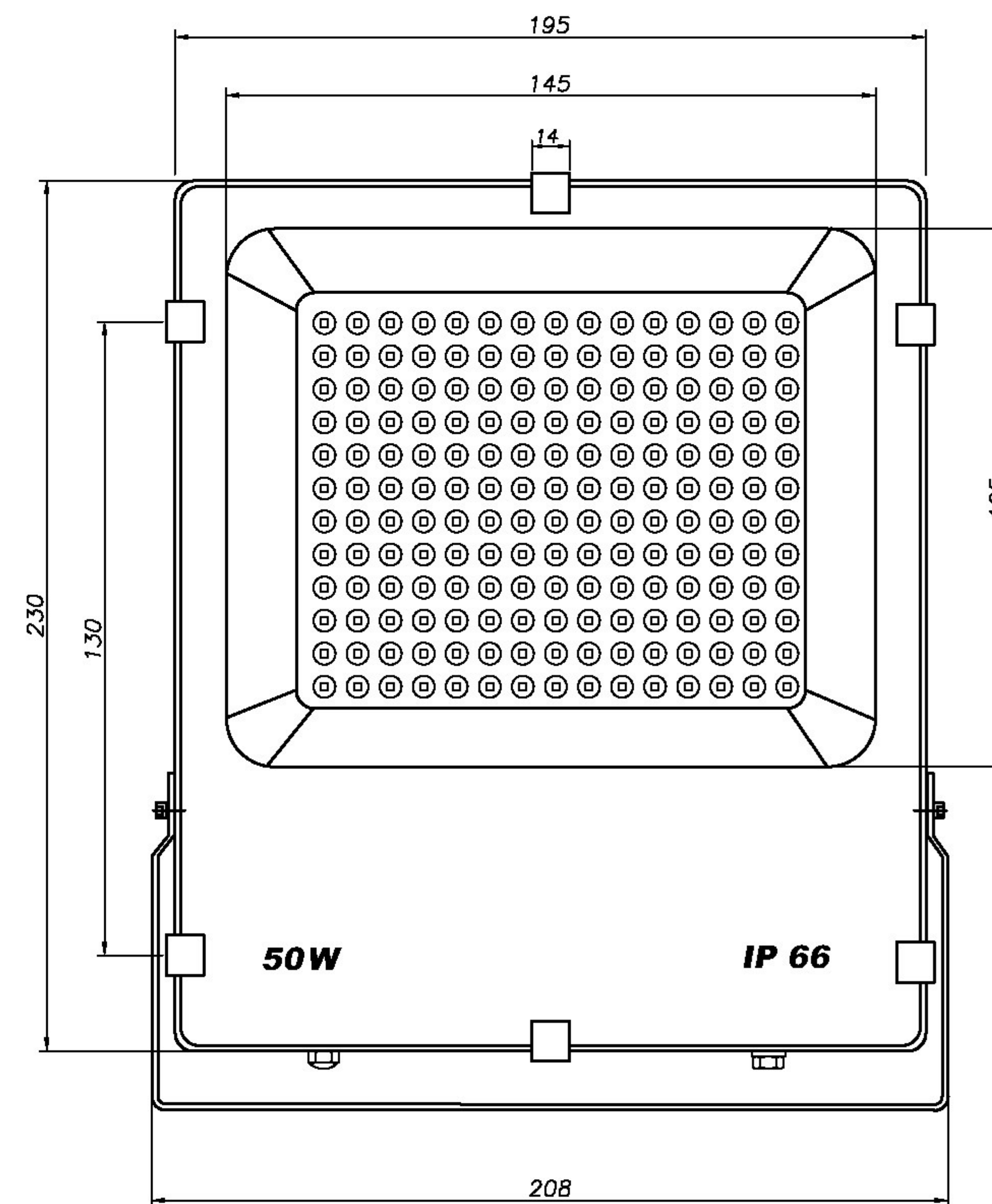
View front
