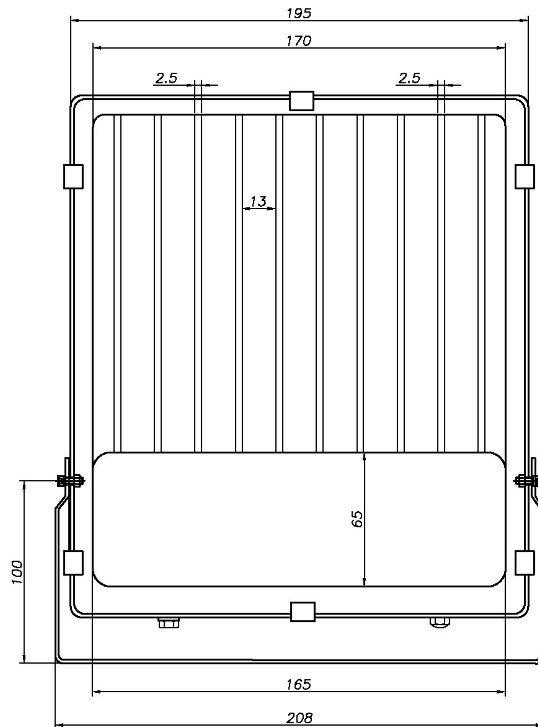
View back
