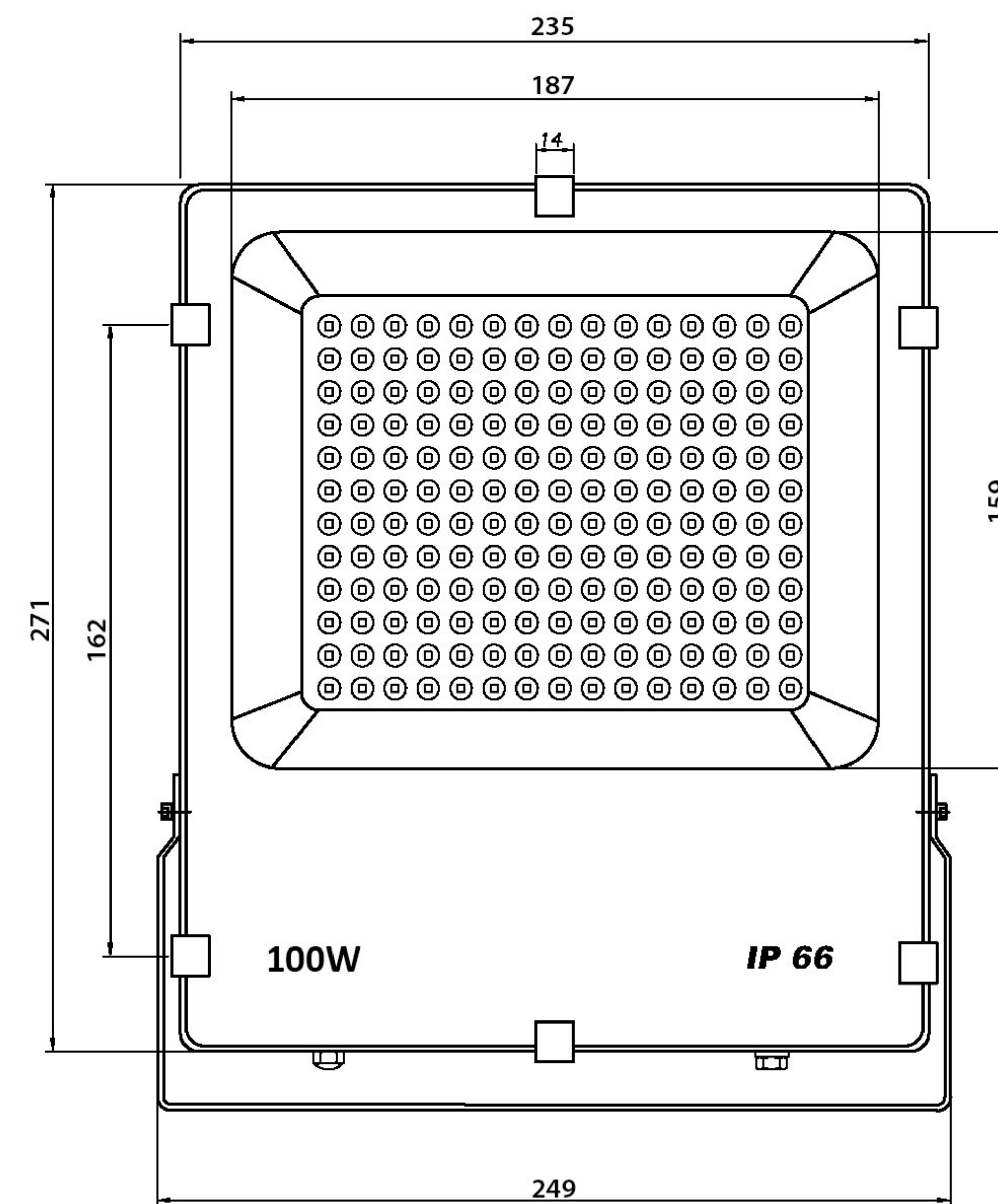
View front
