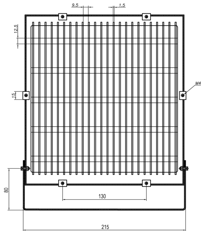
View back
