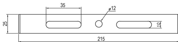
VIEW B
