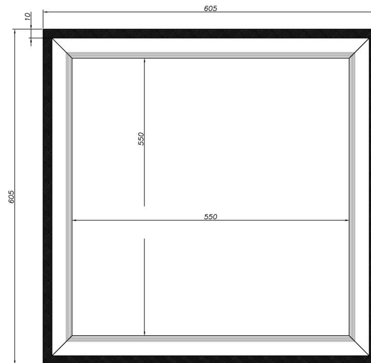
View front
