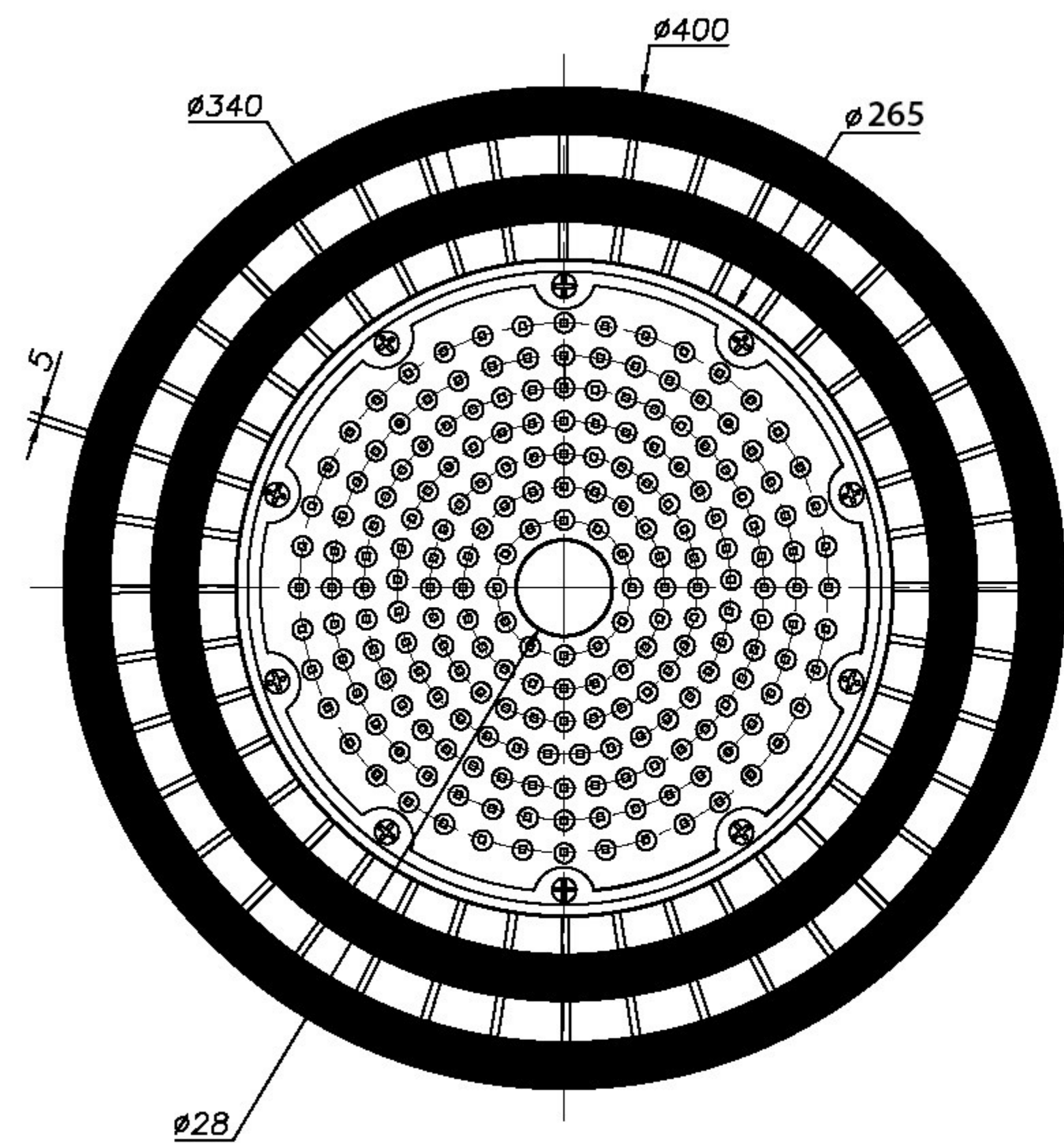
View top
