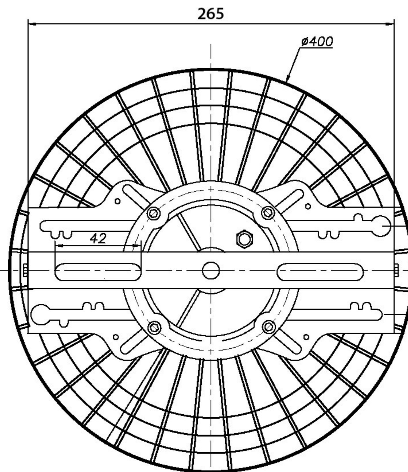
View back
