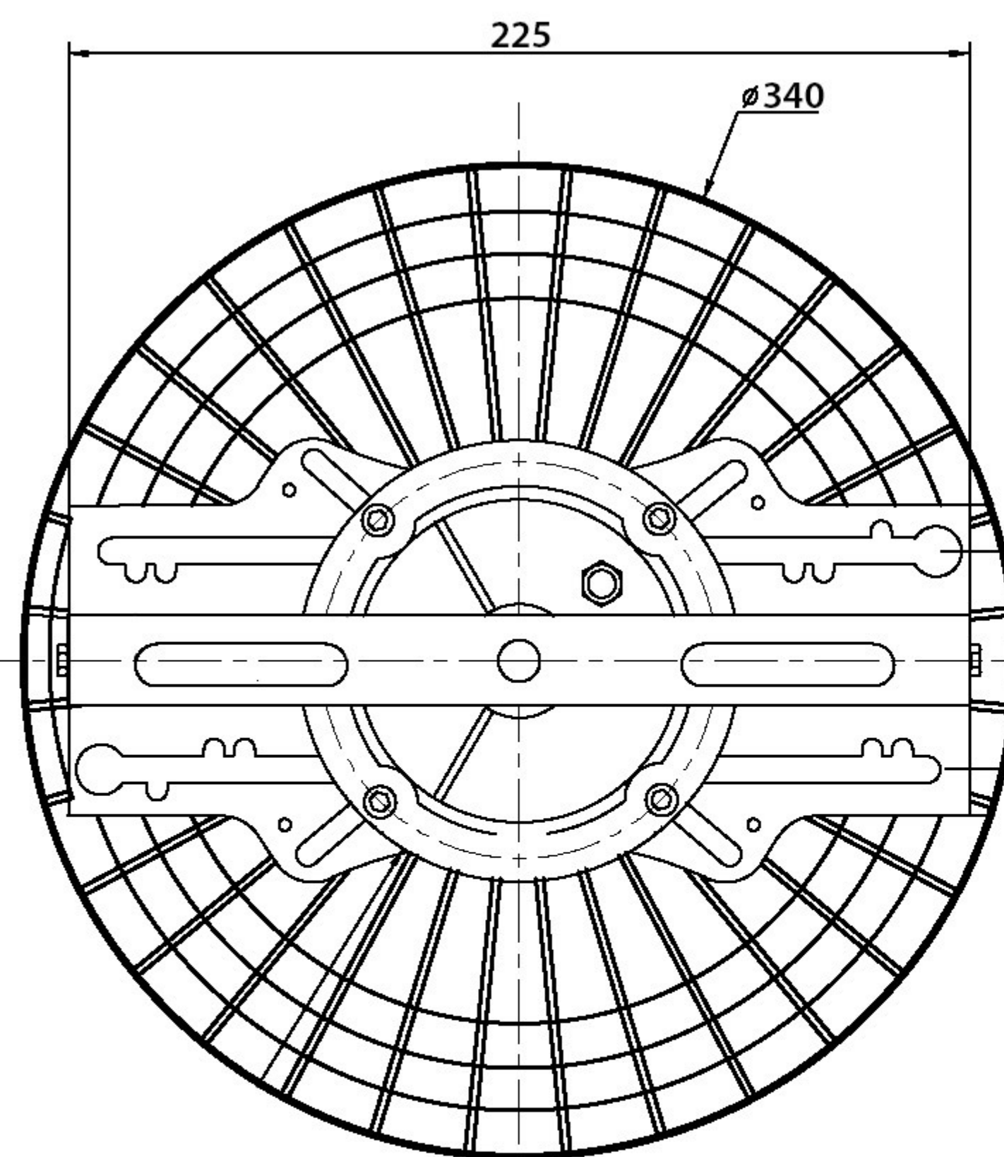
View back
