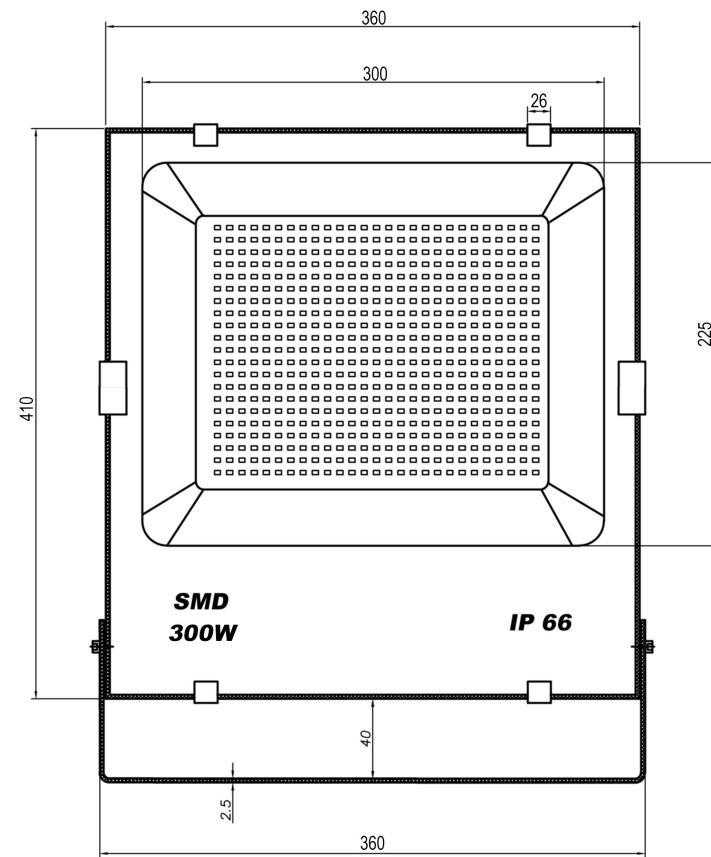
View front
