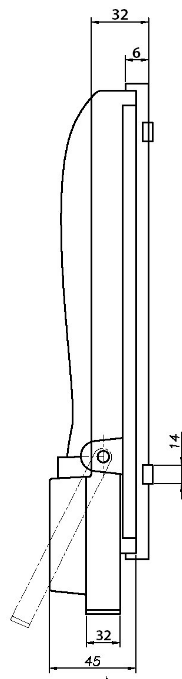
View right
