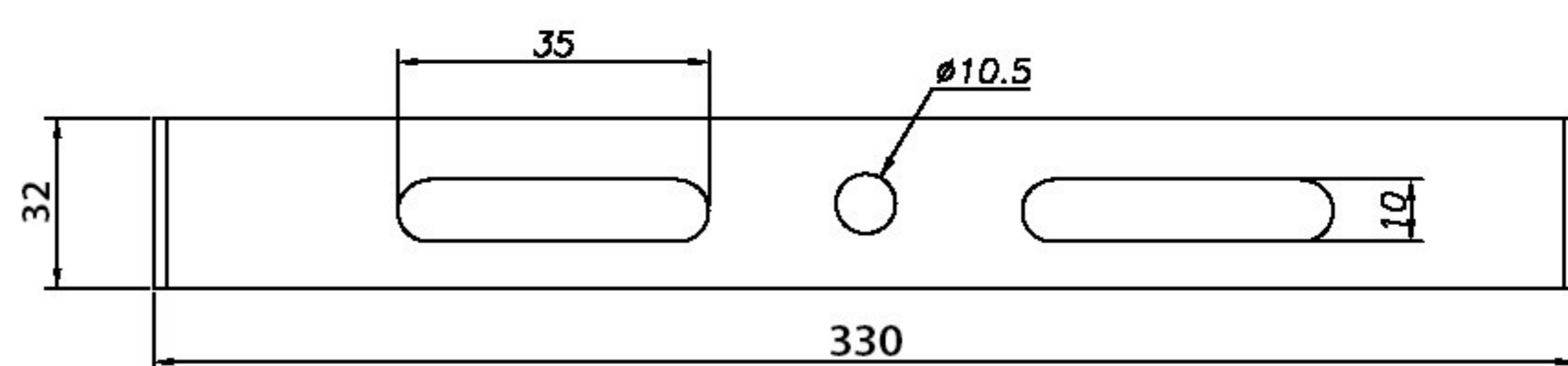
VIEW B
