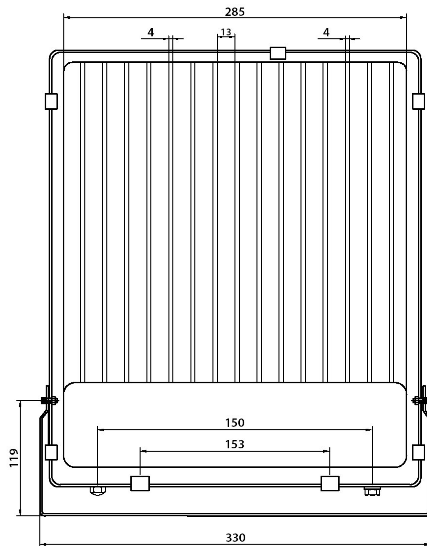
View back
