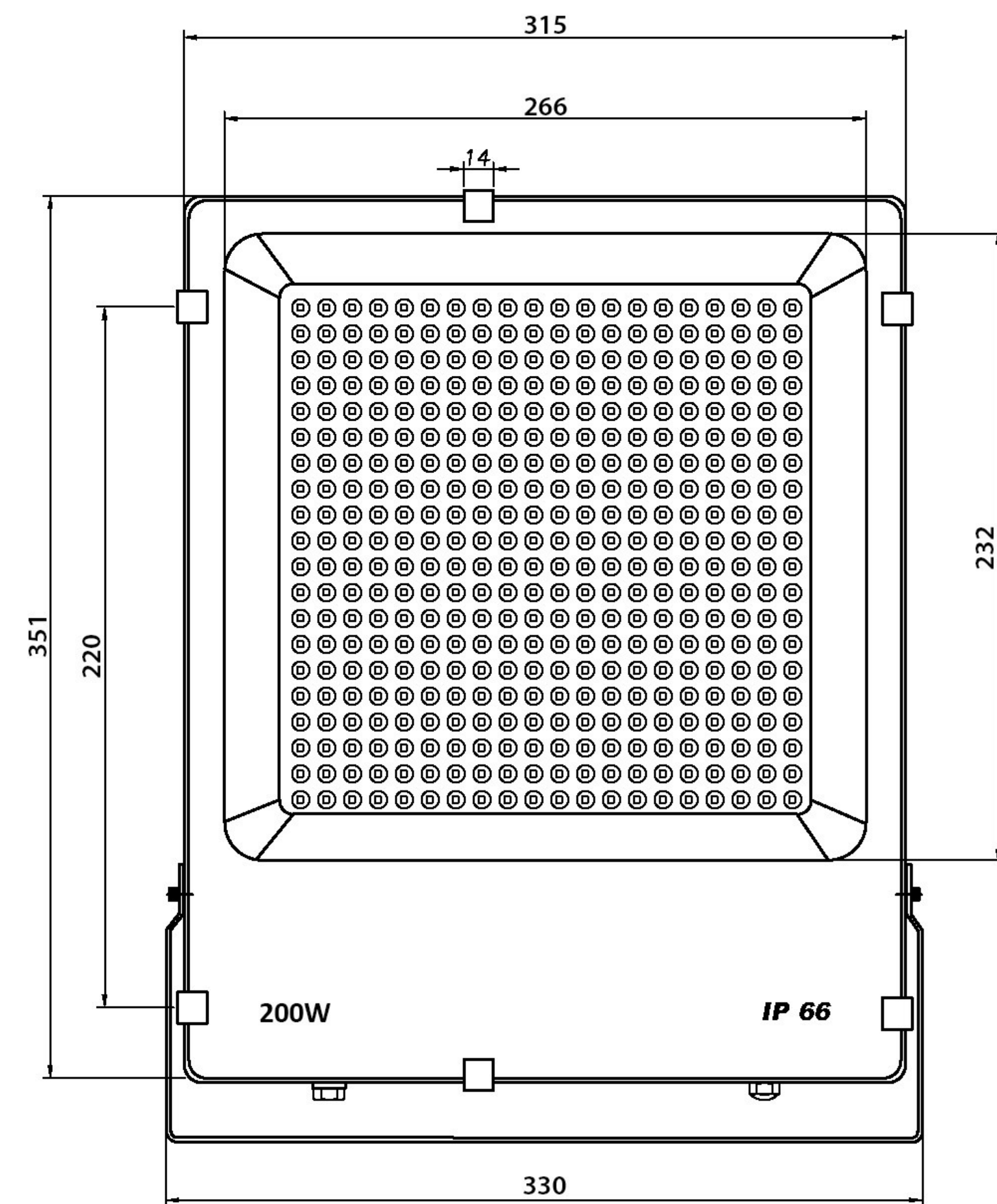
View front
