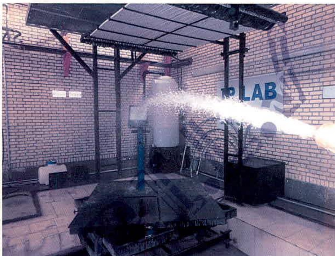
Figure 3: EUT under IPX6
