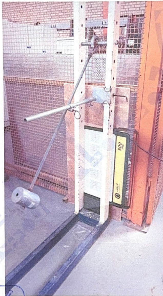
Figure 2: EUT under IK10
